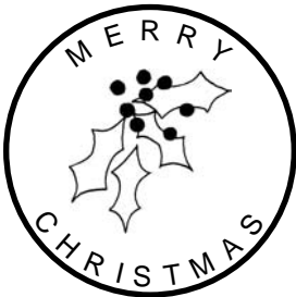
CH3
